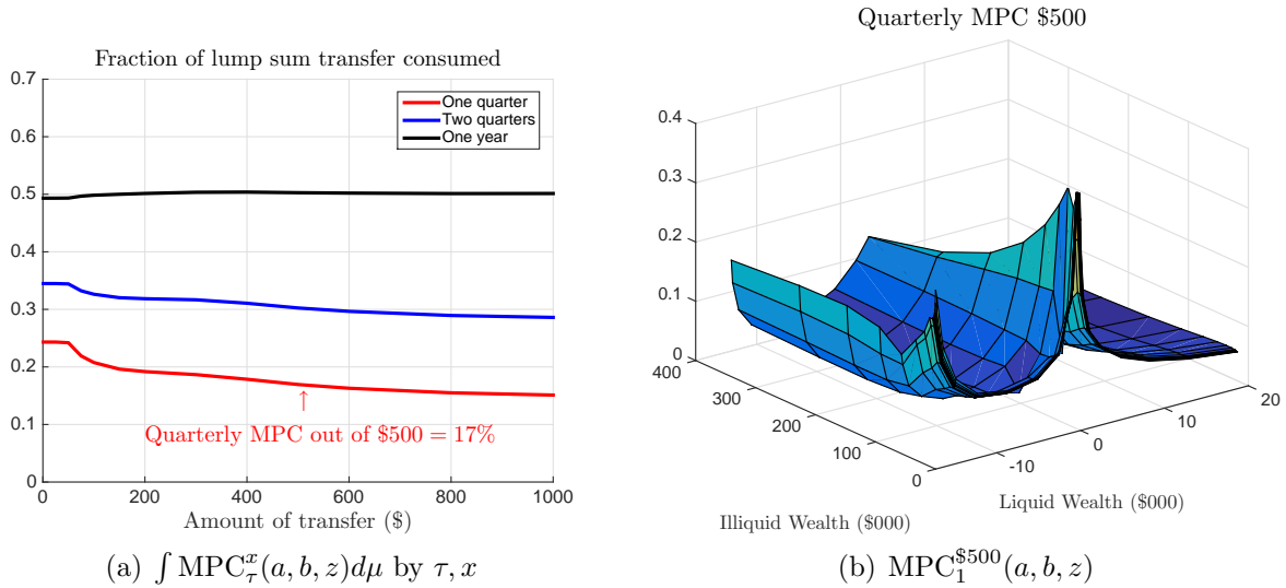
Figure 2: MPC Heterogeneity
